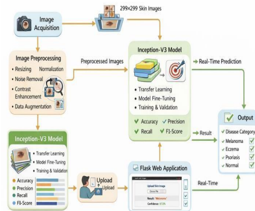
Figure 2: Training and Validation the proposed model
